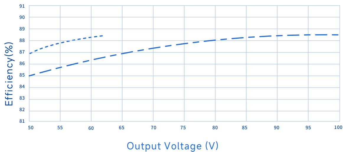
Efficiency Vs. Output Voltage(Vin=220Vac)
